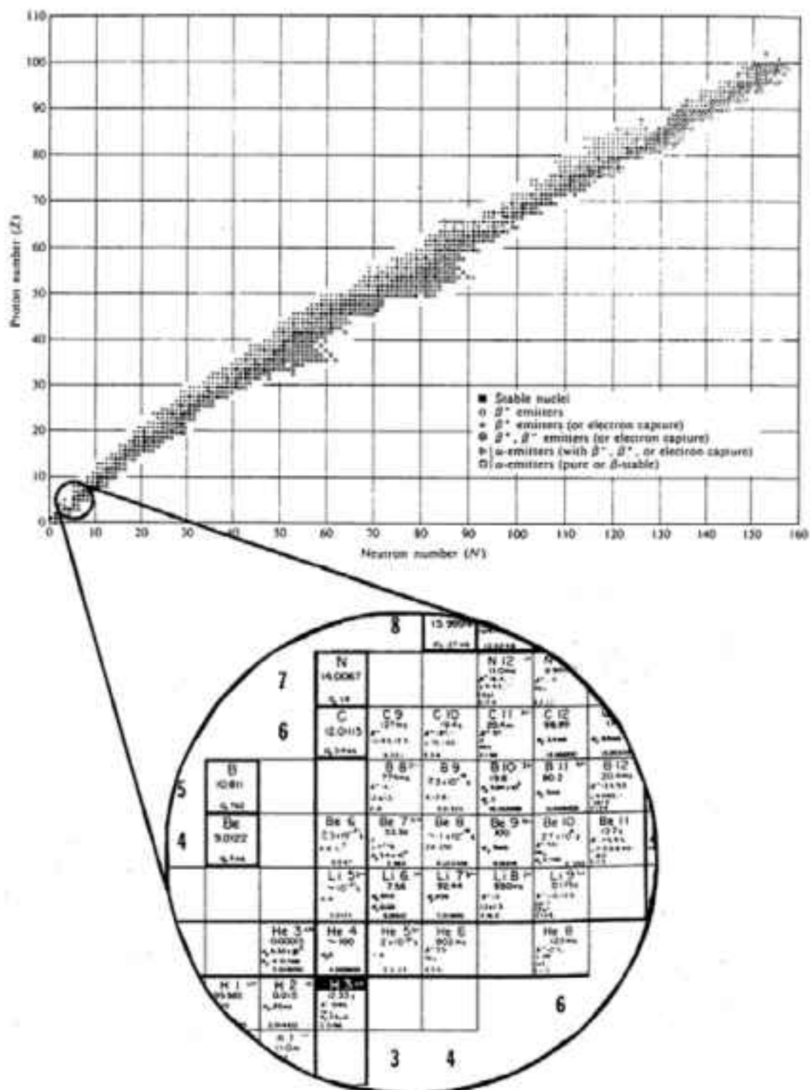
FIG. 3. Chart of radionuclides
