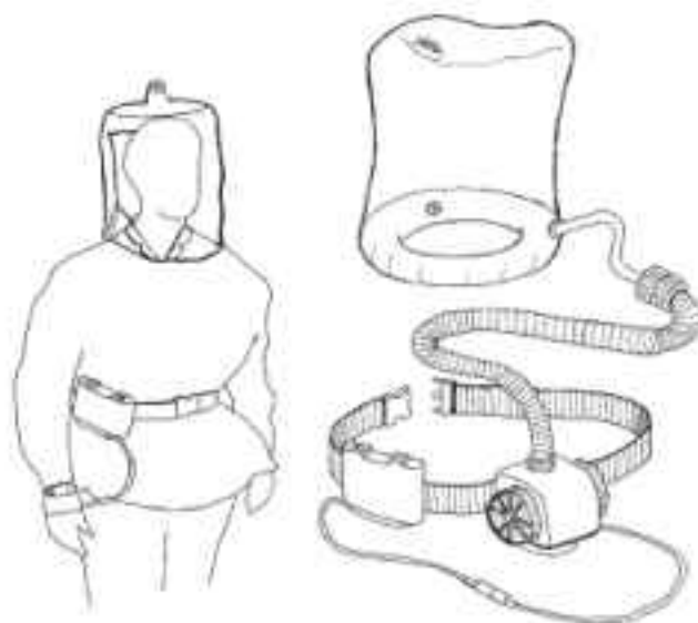
FIG. 36. Powered hood and blouses
