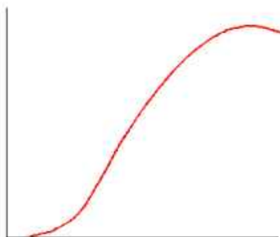
FIG. 8. Deterministic effects
