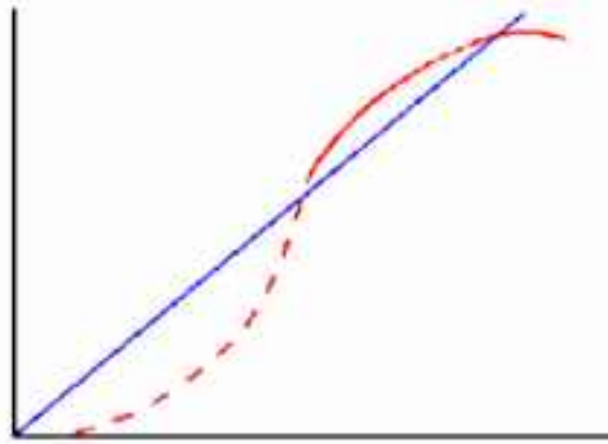
FIG. 9. Stochastic effects
