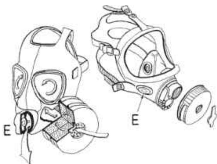
FIG. 33. Full face mask respirators with visor or individual eyepieces
